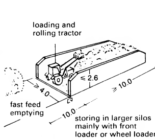
10 Flat silo
